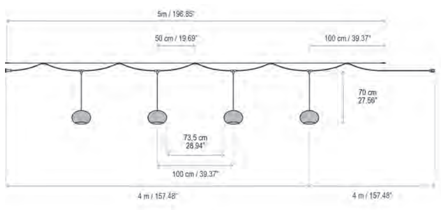
Garota Catenary S/27/4L IP-66
